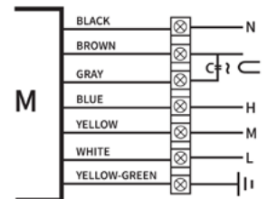
VFM190-3 B2M190-70-3 Three speed wiring
