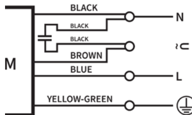
VFM190-1 B2M190-70 Single speed wiring
