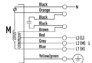
VWM190-3 B2M190-70-3 Three speed wiring
