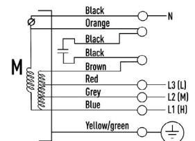
VWM190-3 B2M190-70-3 Three speed wiring
