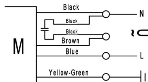
VCM190-1 B2M190-70 Single speed wiring
