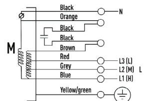
VCM190-1 B2M190-70 Single speed wiring
